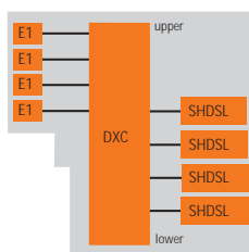
▼ CROCUS SHDSL QUAD SCHEMATIC VIEW
